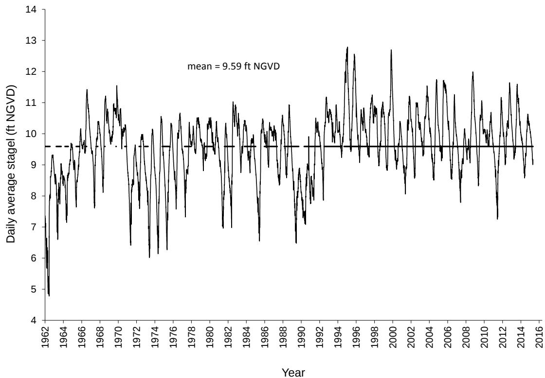
Figure 12. Daily average stage for Water Conservation Area 3A (site CA3AVG).
