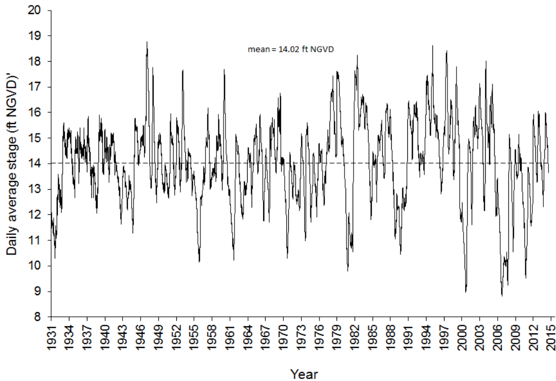
Figure 9. Daily average stage for Lake Okeechobee.
