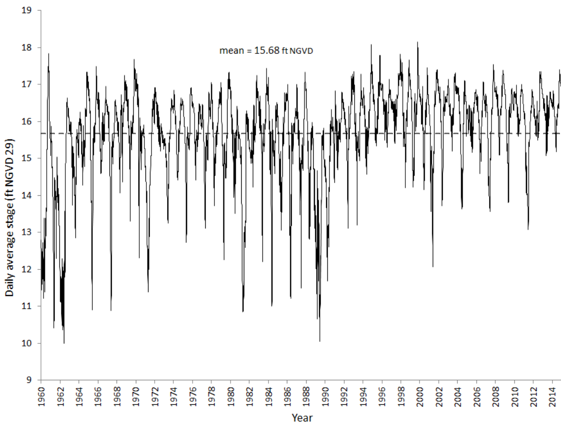
Figure 10. Daily average stage for Water Conservation Area 1 (sites 1-8C, 1-7, 1-8T, and 1-9).
