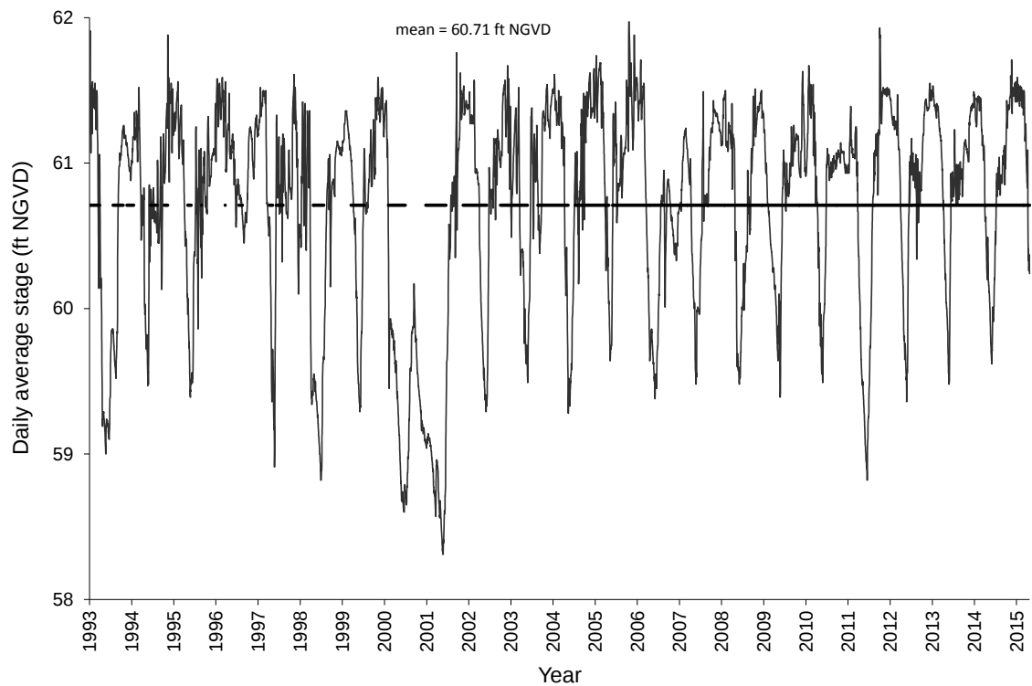
Figure 4. Daily average stage for Lake Gentry (site S63_H).
