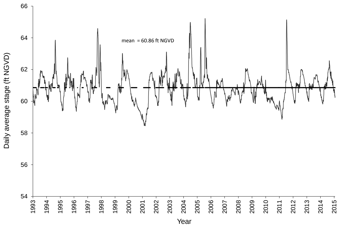
Figure 2. Daily average stage for Lake Myrtle (site S57_H).
