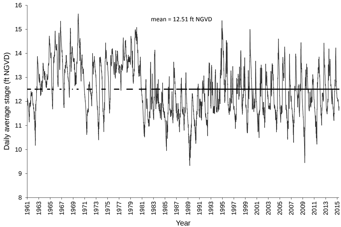
Figure 11. Daily average stage for Water Conservation Area 2A (site 2-17).
