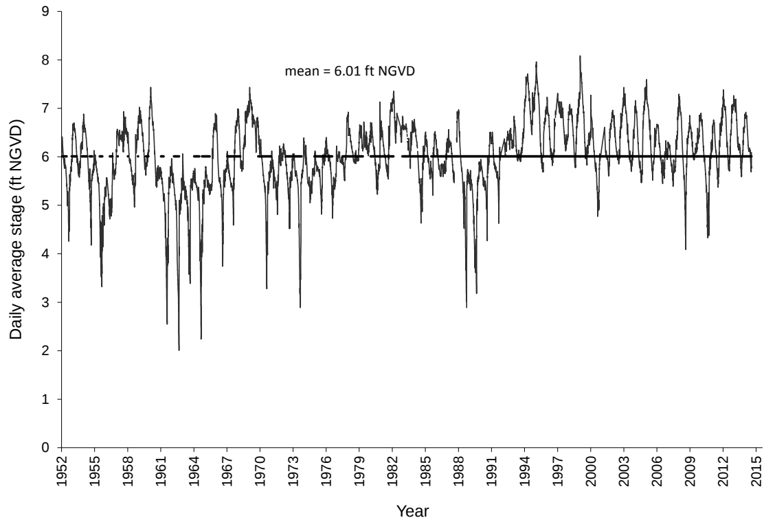
Figure 13. Daily average stage for Everglades National Park (site P-33).
