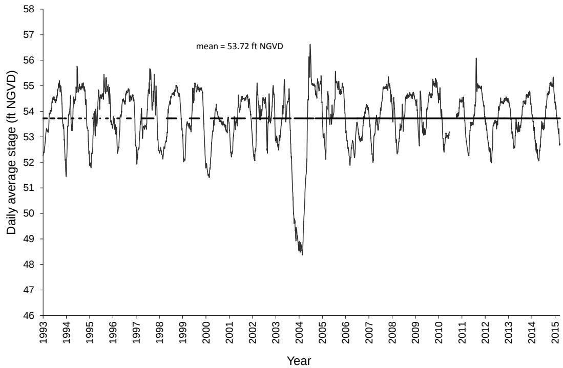
Figure 6. Daily average stage for Lake Tohopekaliga (site S61_H).
