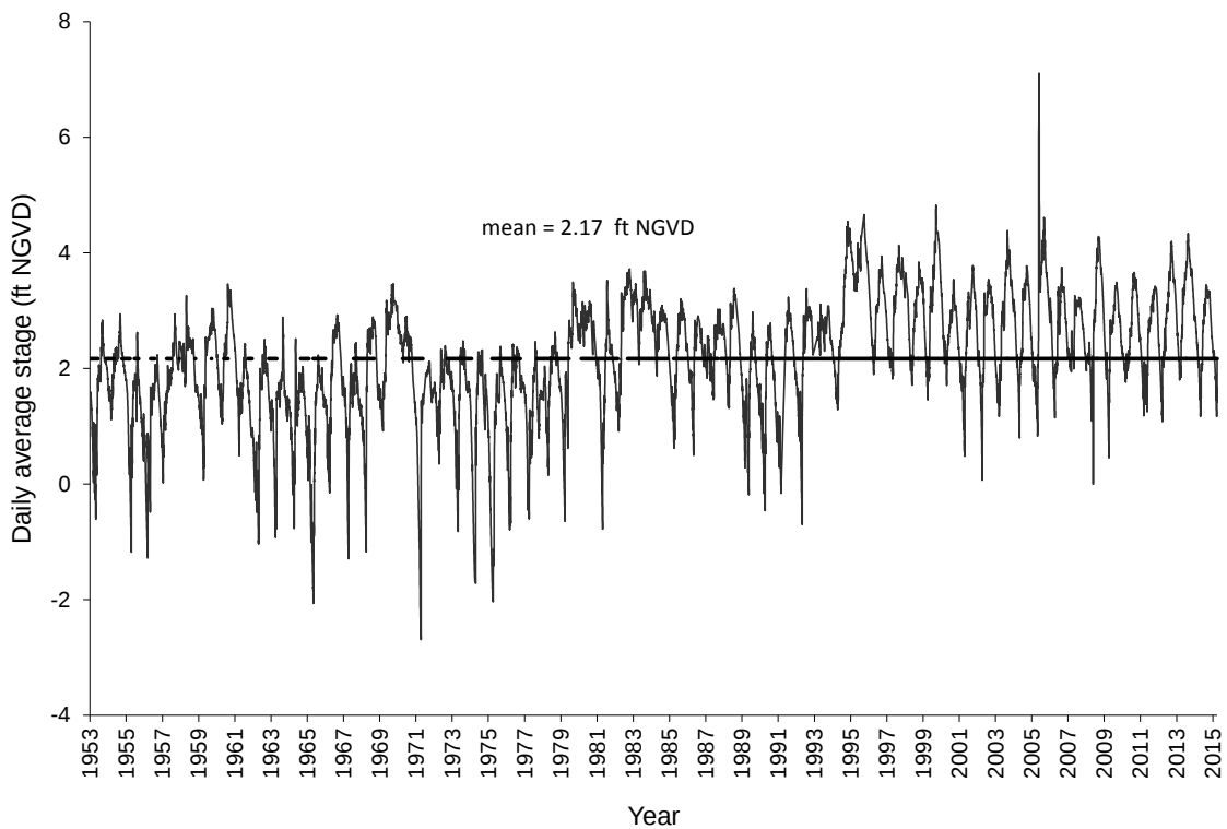
Figure 14. Daily average stage for the Everglades National Park (site P-34).
