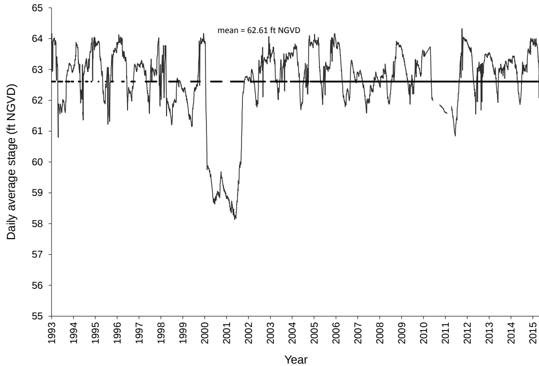
Figure 1. Daily average stage for Lake Alligator (site S60_H). [Note: ft NGVD – feet National Geodetic Vertical Datum of 1929.]
