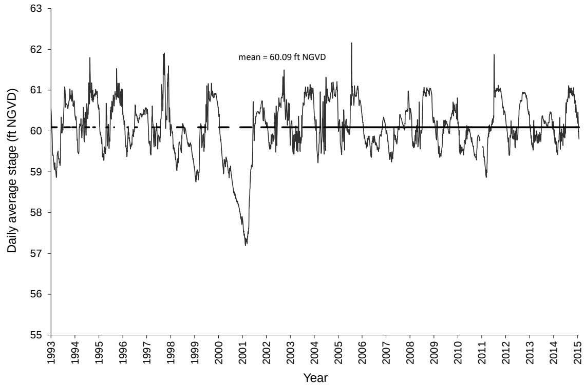
Figure 3. Daily average stage for Lake Mary Jane (site S62_H).
