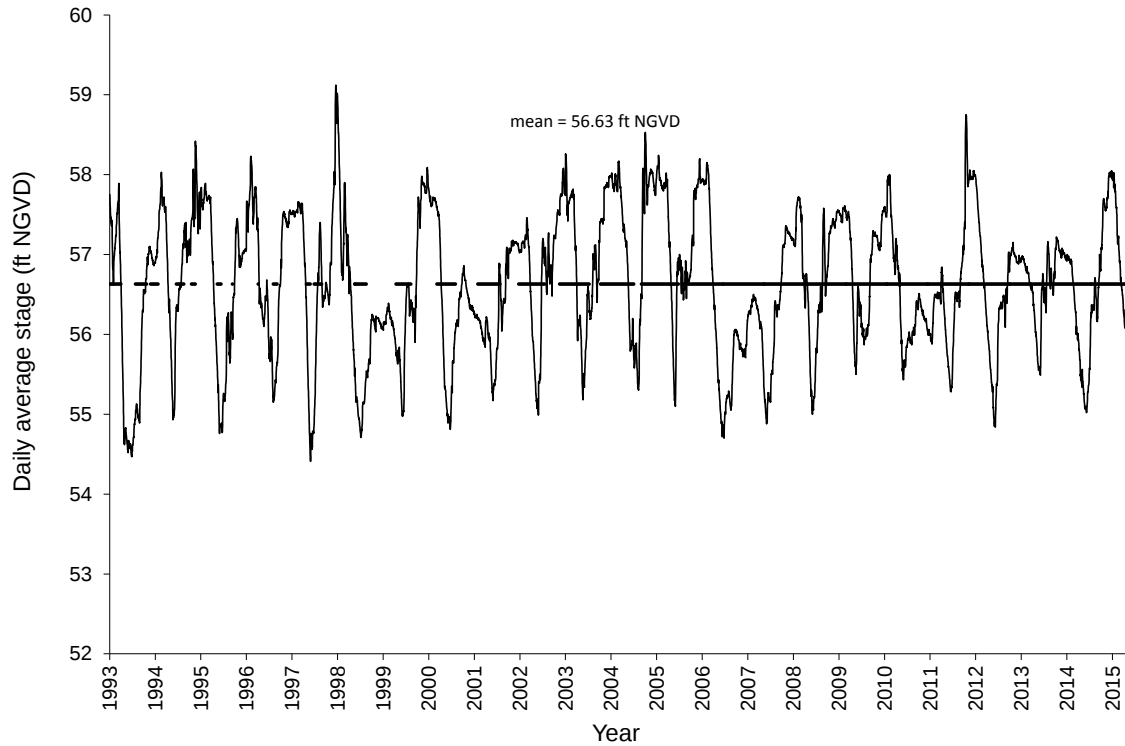
Figure 5. Daily average stage for East Lake Tohopekaliga (site S59_H).
