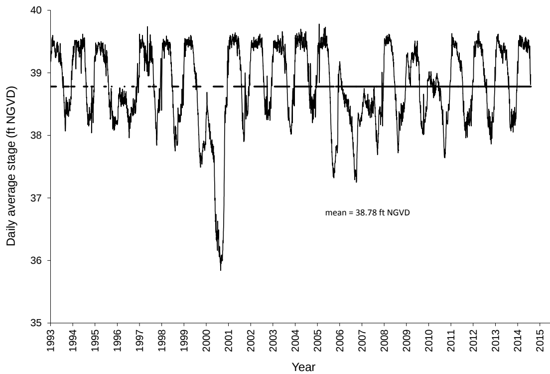
Figure 8. Daily average stage for Lake Istokpoga (site S68_H).
