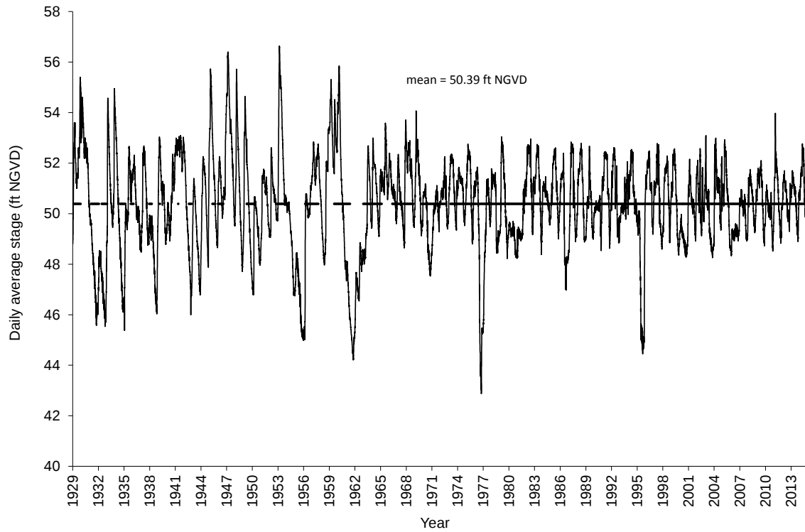
Figure 7. Daily average stage for Lake Kissimmee (site S65_H).
