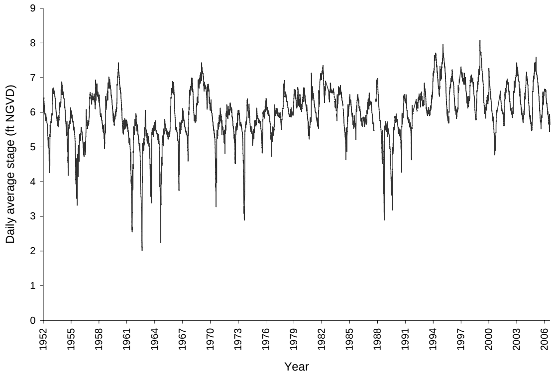
Figure 13. Daily average stage for Everglades National Park at site P33.
