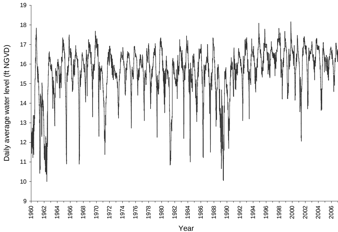
Figure 10. Daily average stage for Water Conservation Area 1.
