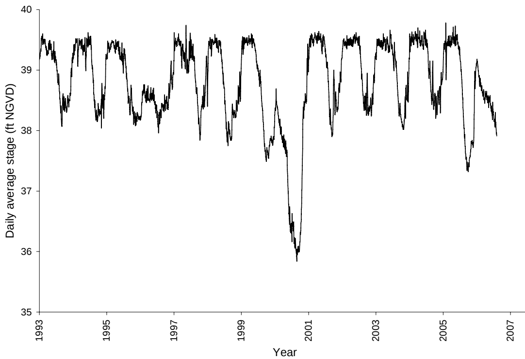
Figure 8. Daily average stage for Lake Istokpoga.
