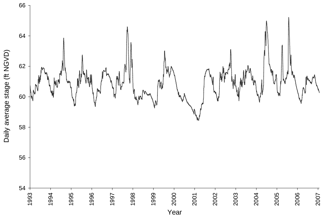
Figure 2. Daily average stage for Lake Myrtle.
