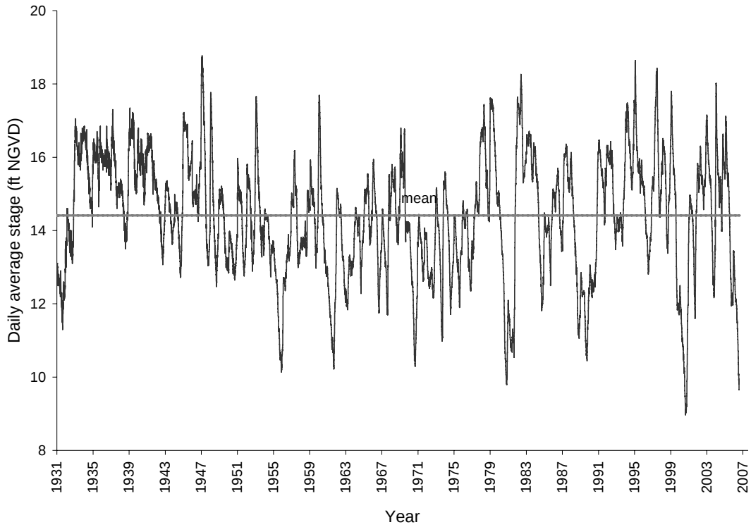
Figure 9. Daily average stage for Lake Okeechobee.
