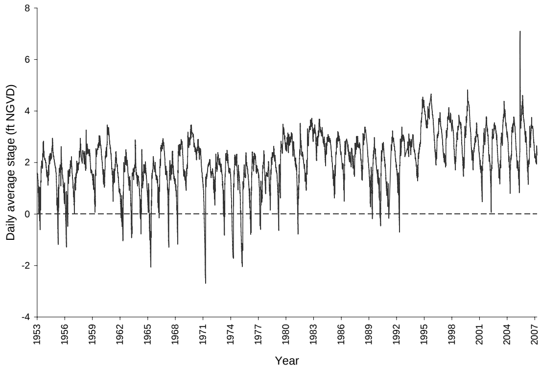
Figure 14. Daily average stage for Everglades National Park at site P34.
