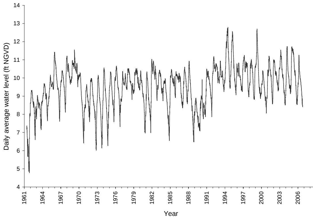
Figure 12. Daily average stage for Water Conservation Area 3A.
