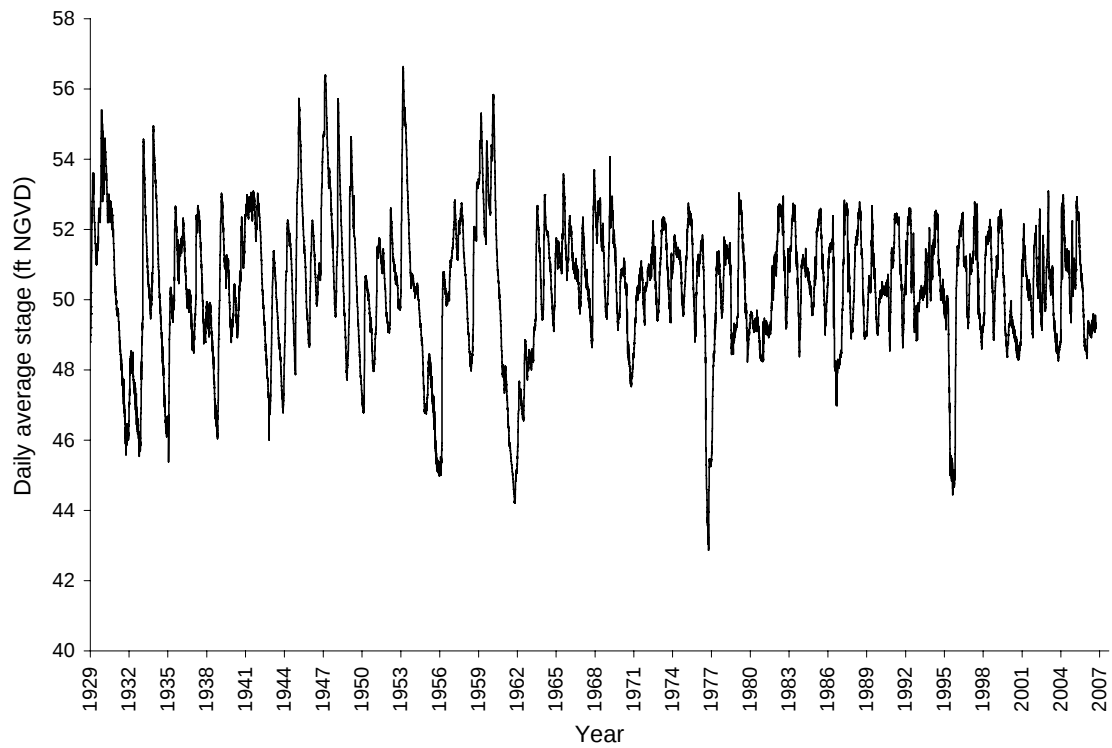
Figure 7. Daily average stage for Lake Kissimmee.
