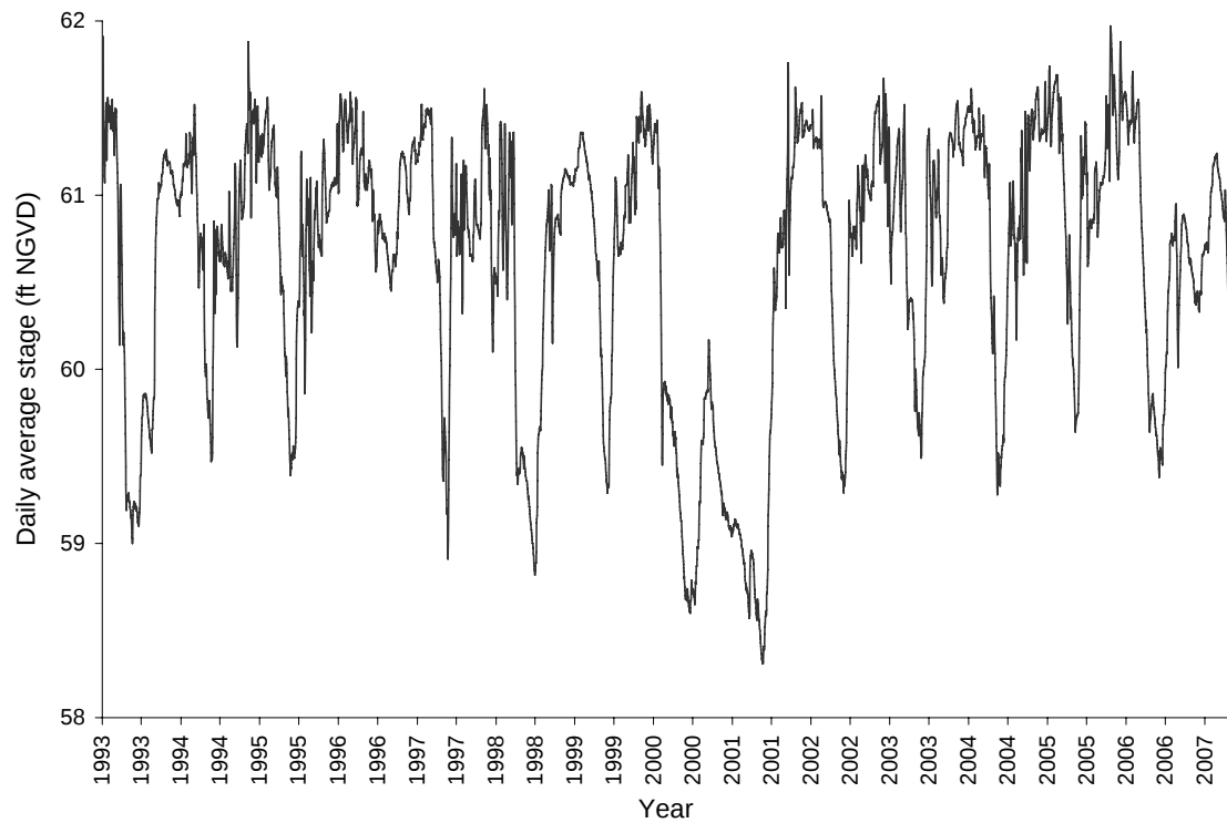
Figure 4. Daily average stage for Lake Gentry.
