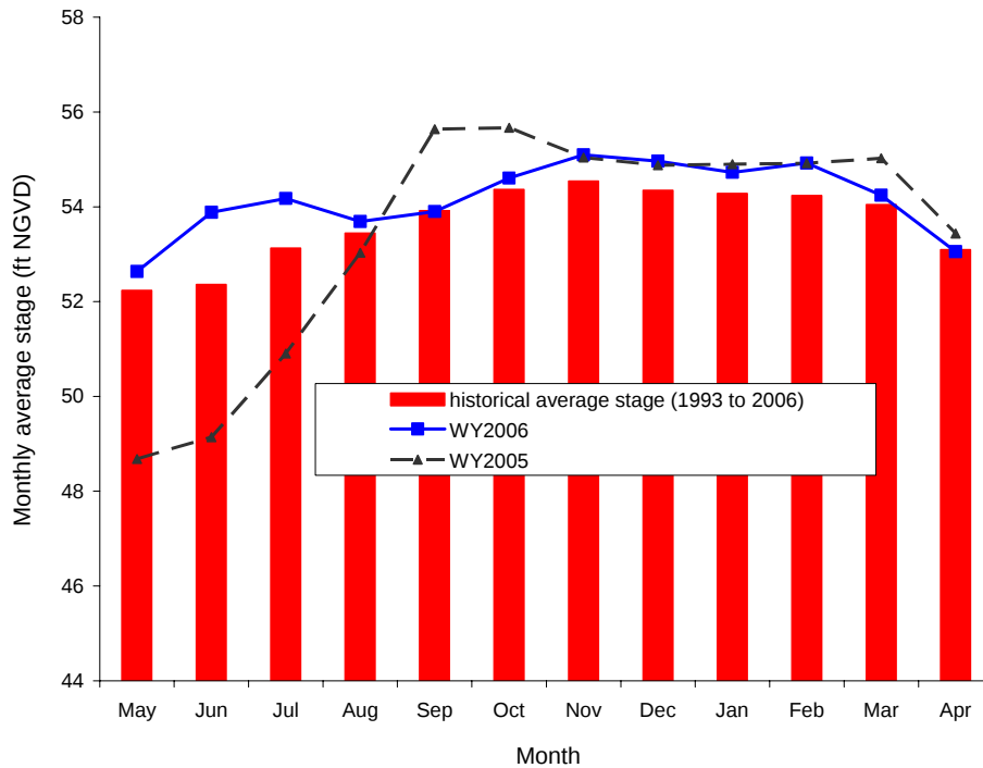
Figure 6. Monthly average water levels for Lake Tohopekaliga (site S61_H).
