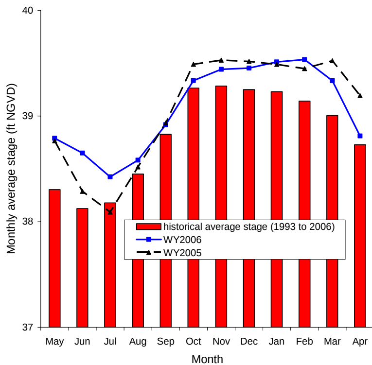
Figure 8. Monthly average water levels for Lake Istokpoga (site S68_H).
