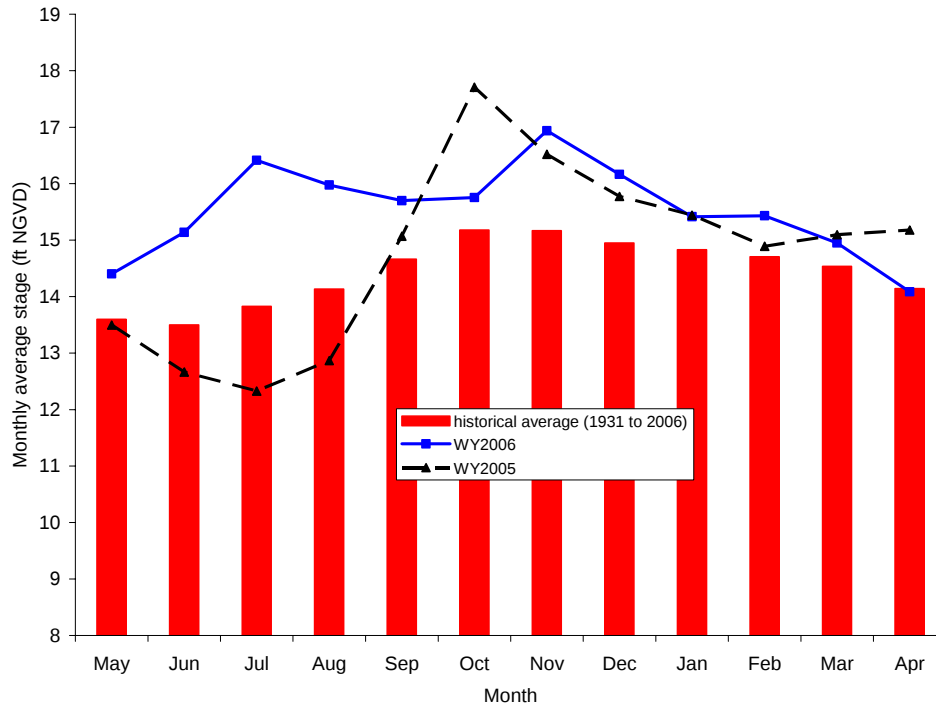
Figure 9. Monthly average water levels for Lake Okeechobee.
