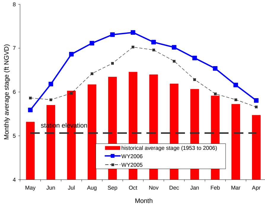
Figure 13. Monthly average water levels for site P-33 in the ENP.
