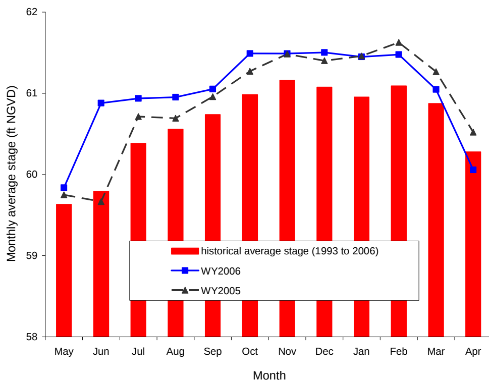
Figure 4. Monthly average water levels for Lake Gentry (site S63_H).
