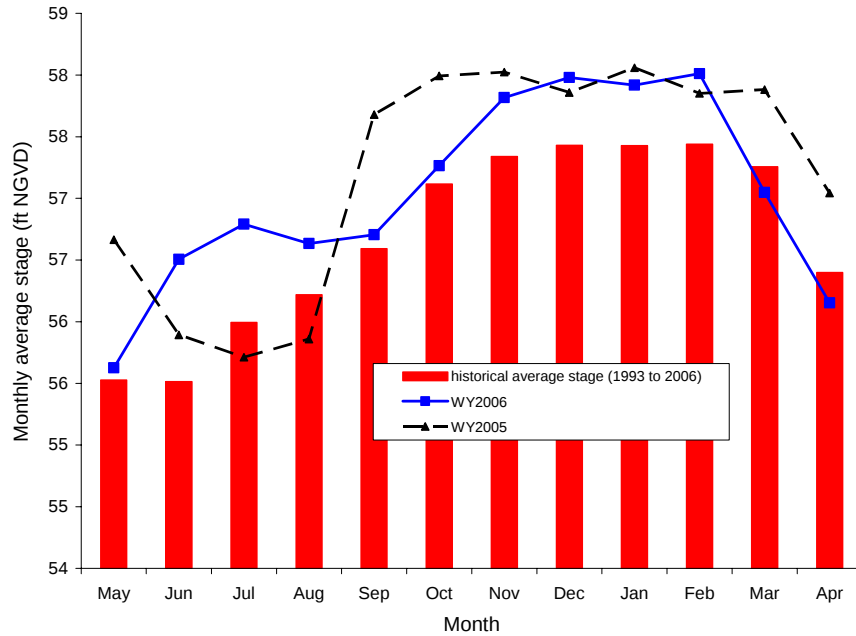
Figure 5. Monthly average water levels for East Lake Tohopekaliga (site S59_H).
