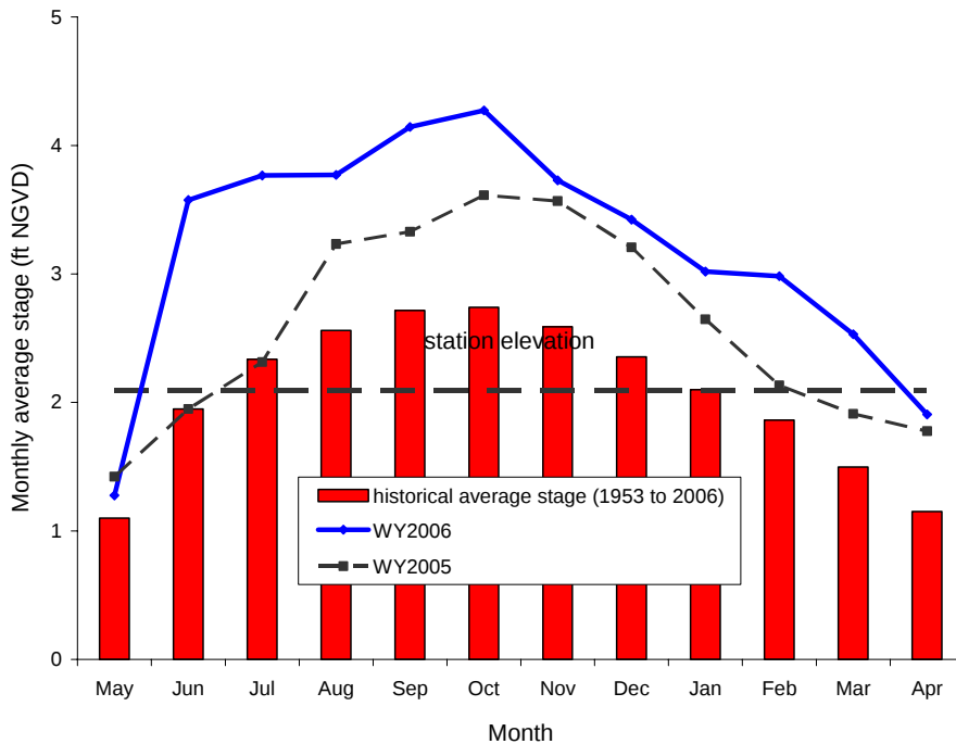
Figure 14. Monthly average water levels for site P-34 in the ENP.
