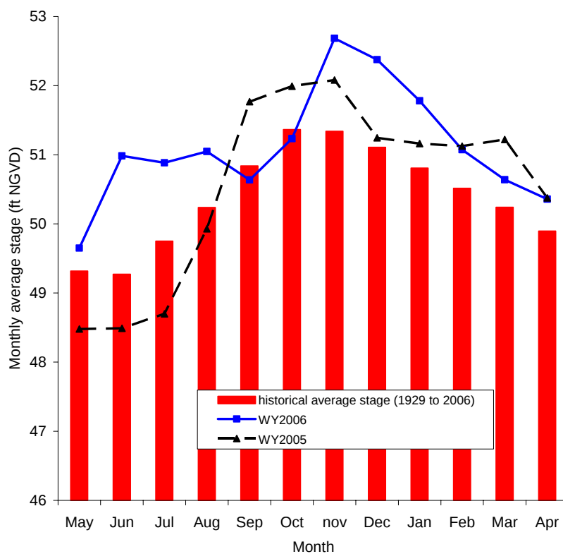
Figure 7. Monthly average water levels for Lake Kissimmee (S65_H).
