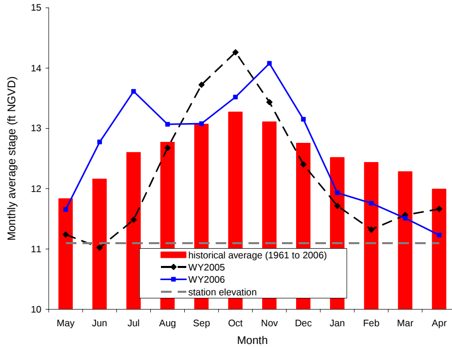
Figure 11. Monthly average water levels for WCA-2A (site 2-17).
