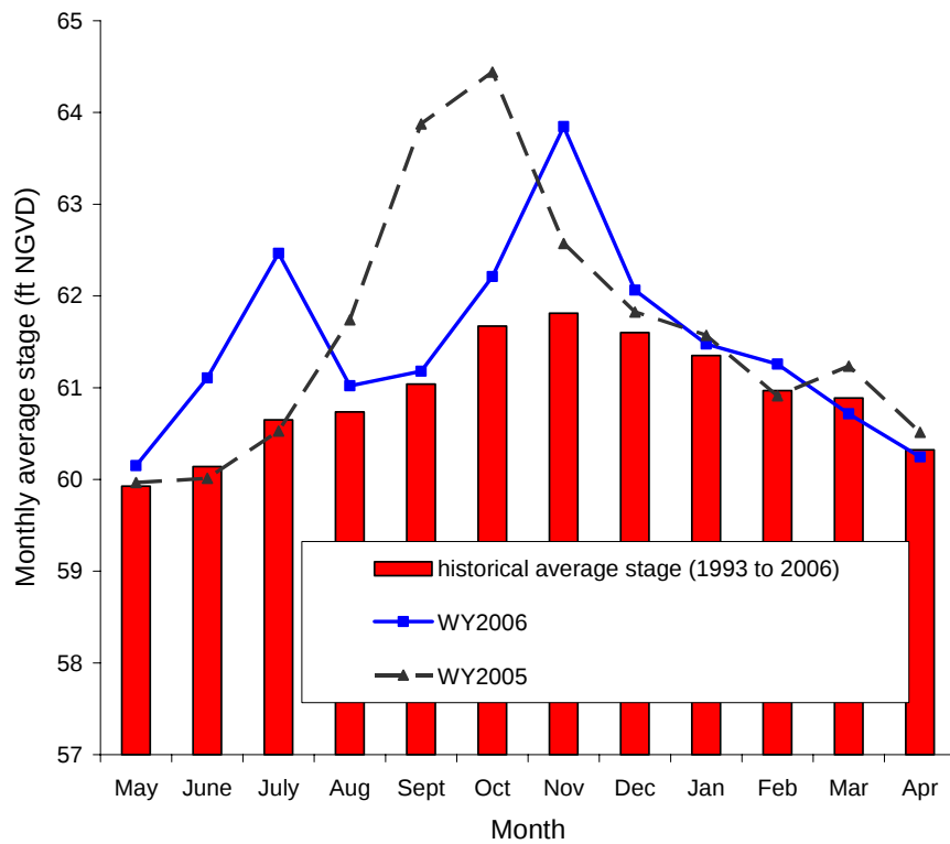
Figure 2. Monthly average water levels for Lake Myrtle (site S57_H).
