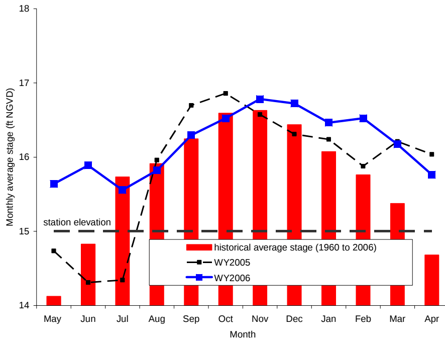
Figure 10. Monthly average water levels for WCA-1 (sites 1-8C, 1-7, 1-8T, and 1-9).
