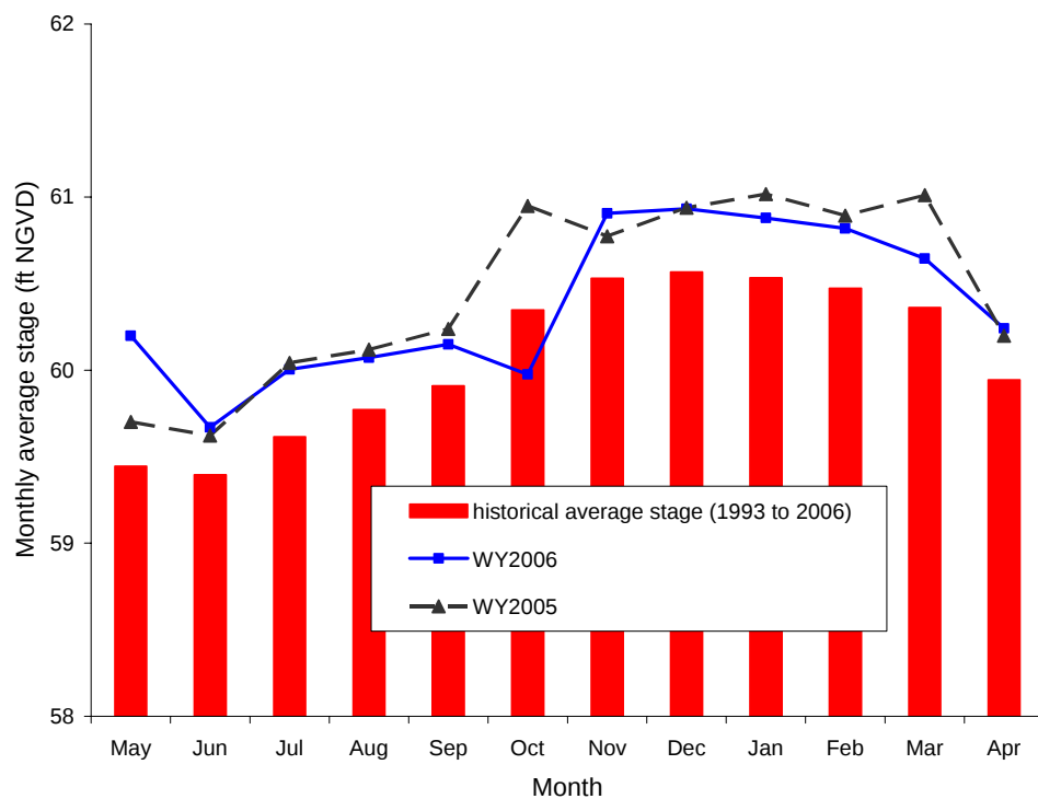
Figure 3. Monthly average water levels for Lake Mary Jane (site S62_H).
