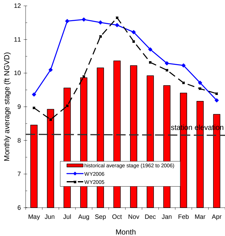
Figure 12. Monthly average water levels for WCA-3A (CA3AVG).
