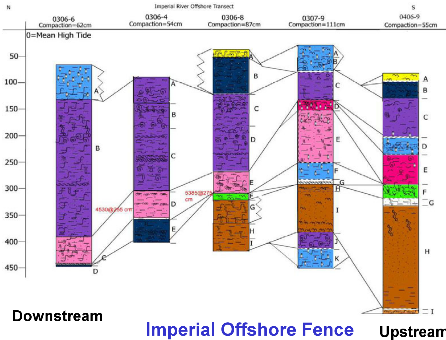
Figure 31. Fence diagram for the offshore transect of the Imperial River. Cores are oriented, from left to right, downstream (north) to upstream (south). Facies color-codes same as in Figure 28.
