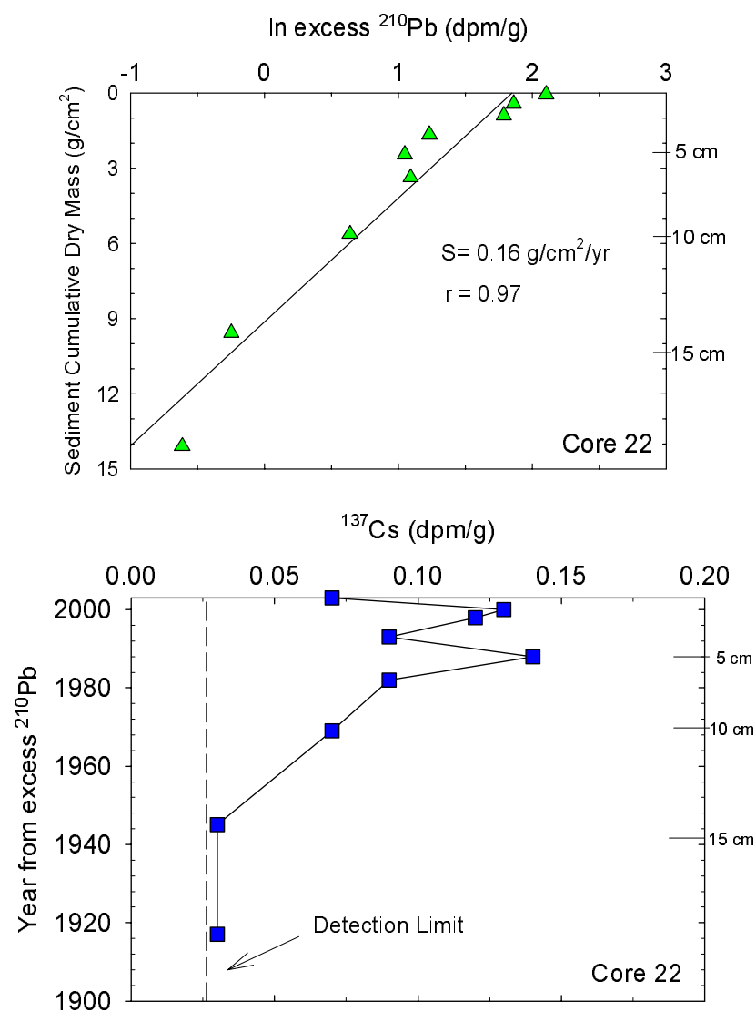
Figure 45. Vertical profiles for the natural logarithm (ln) of the activity of excess ^{210}\text{Pb} versus cumulative dry mass of sediment (upper graph) and activity of ^{137}\text{Cs} versus year determined from the excess ^{210}\text{Pb} data (CIC model). Right-hand axes show sediment depths in cm. Solid line on upper graph shows best fit linear regression line, S = sediment accumulation rate and r = correlation coefficient. Dashed line on the lower graph shows analytical detection limit for activity of ^{137}\text{Cs} .
