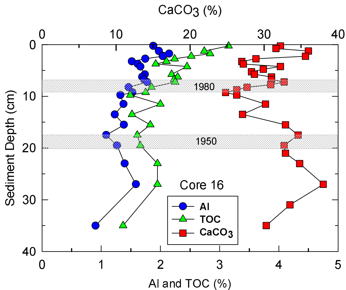
Figure 55. Vertical profiles for concentrations of aluminum (Al), total organic carbon (TOC), and calcium carbonate ( \text{CaCO}_3 ) for sediments for core 16 from Estero Bay. Shaded areas shows depth intervals that corresponds to ~1950 and 1980.
