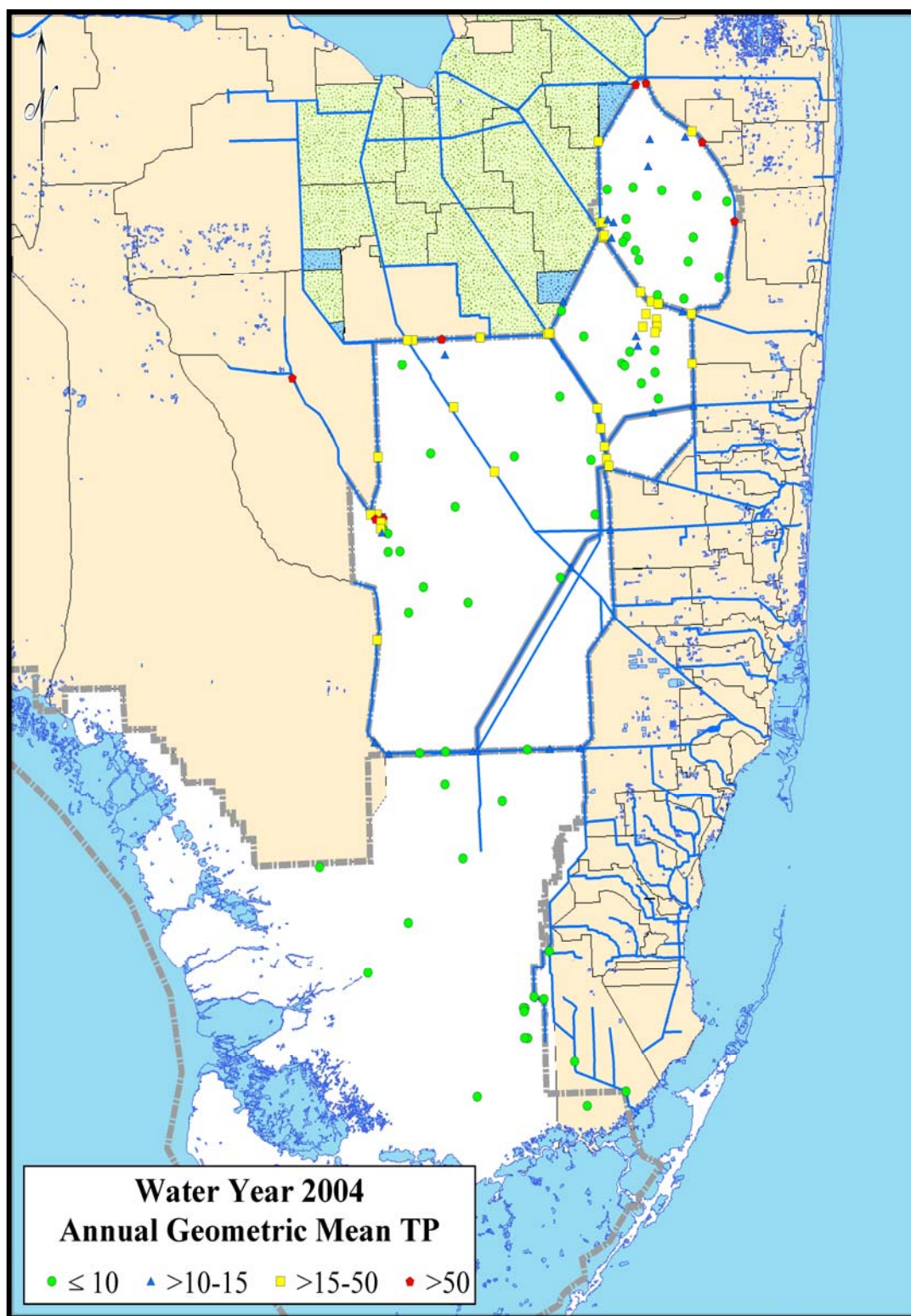
Figure 2C-2. Summary of geometric mean TP concentrations (µg/L) at stations across the EPA for WY2004. Geometric mean TP concentrations are classified utilizing four levels: \leq 10 µg/L, 10–15 µg/L, 15–50 µg/L, and > 50 µg/L.
