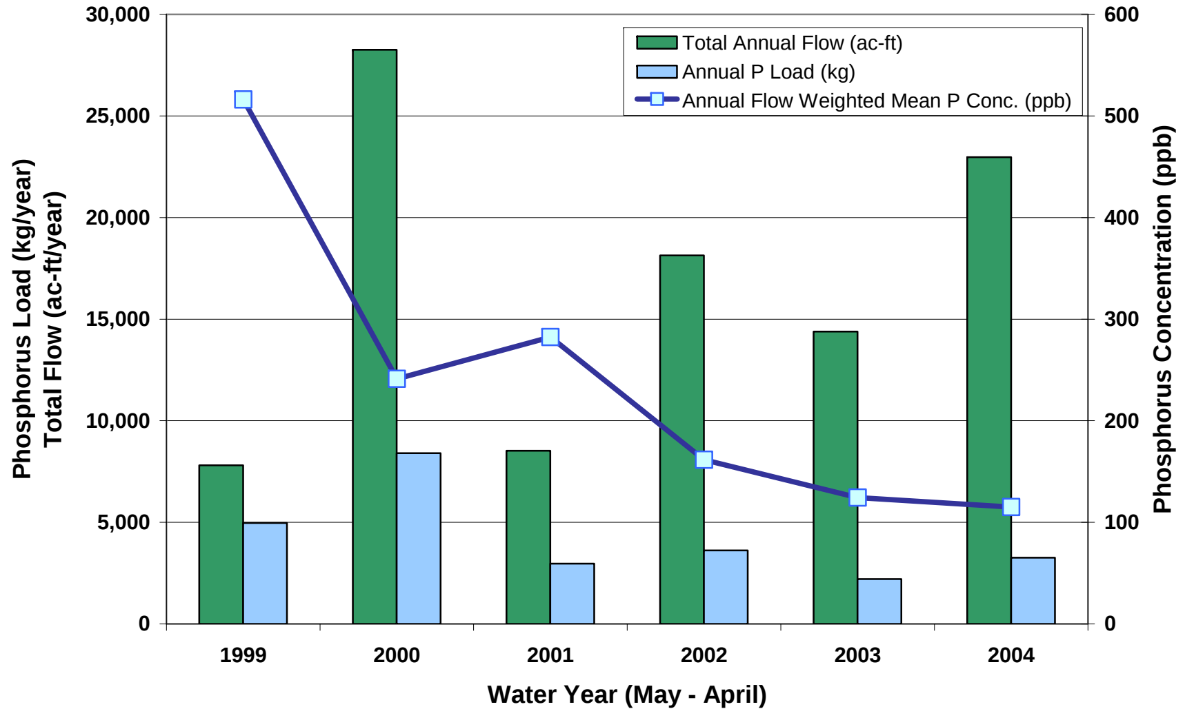
Figure A-5a. Historic summary of TP flows and loads at McDaniel Ranch compliance points.
