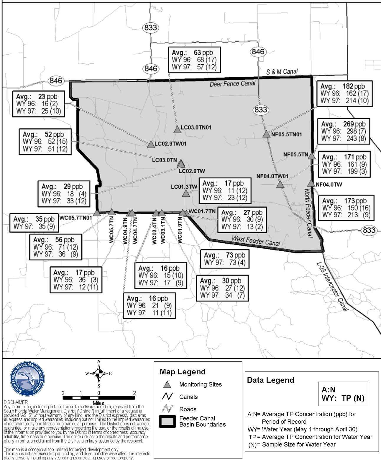
Figure A-5b. Upstream monitoring sites: summary of TP data (ppb).
