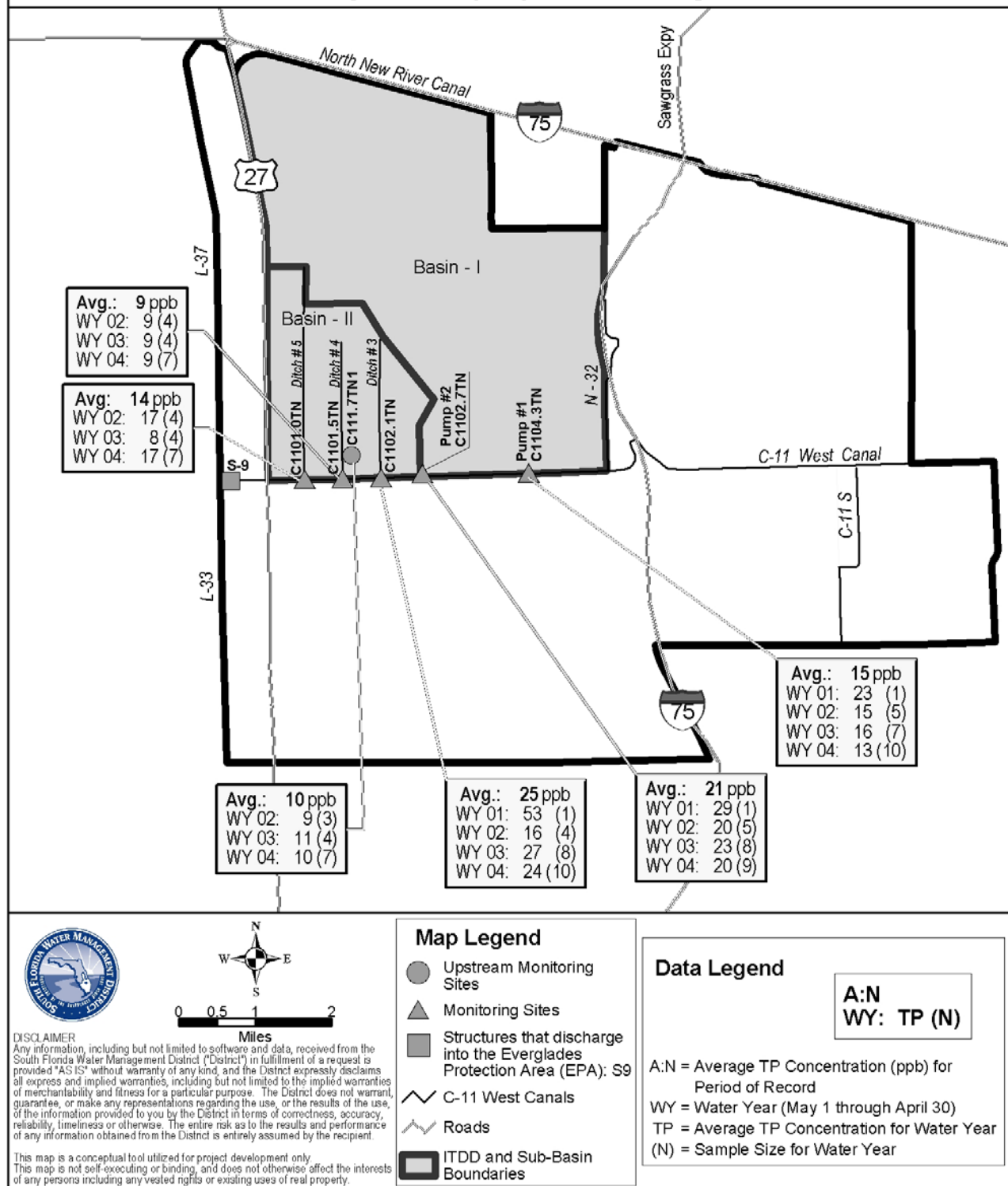
Figure A-3c. Upstream monitoring sites: summary of TP data (ppb).
