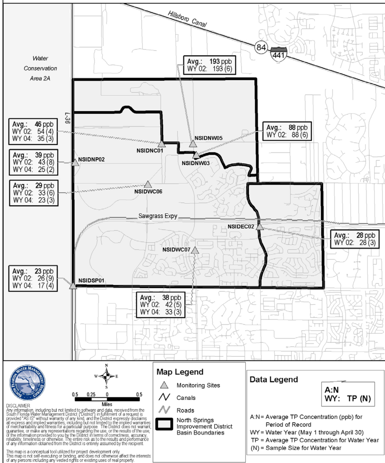
Figure A-2. Upstream monitoring sites: summary of TP data (ppb).
