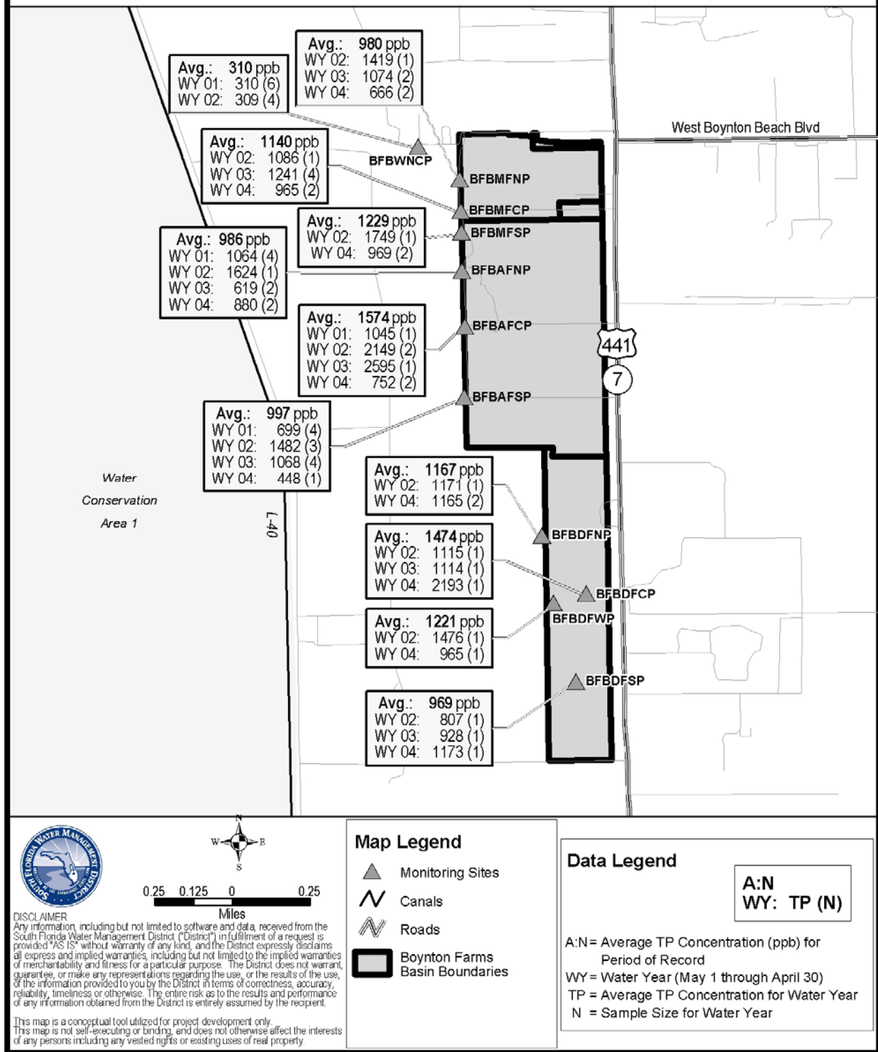
Figure A-7. Summary of TP data (ppb).
